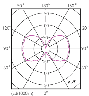
LEDClassic 30W E27 Other Transparent Amber 820 DIM
